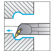
R type insert 117.5°
